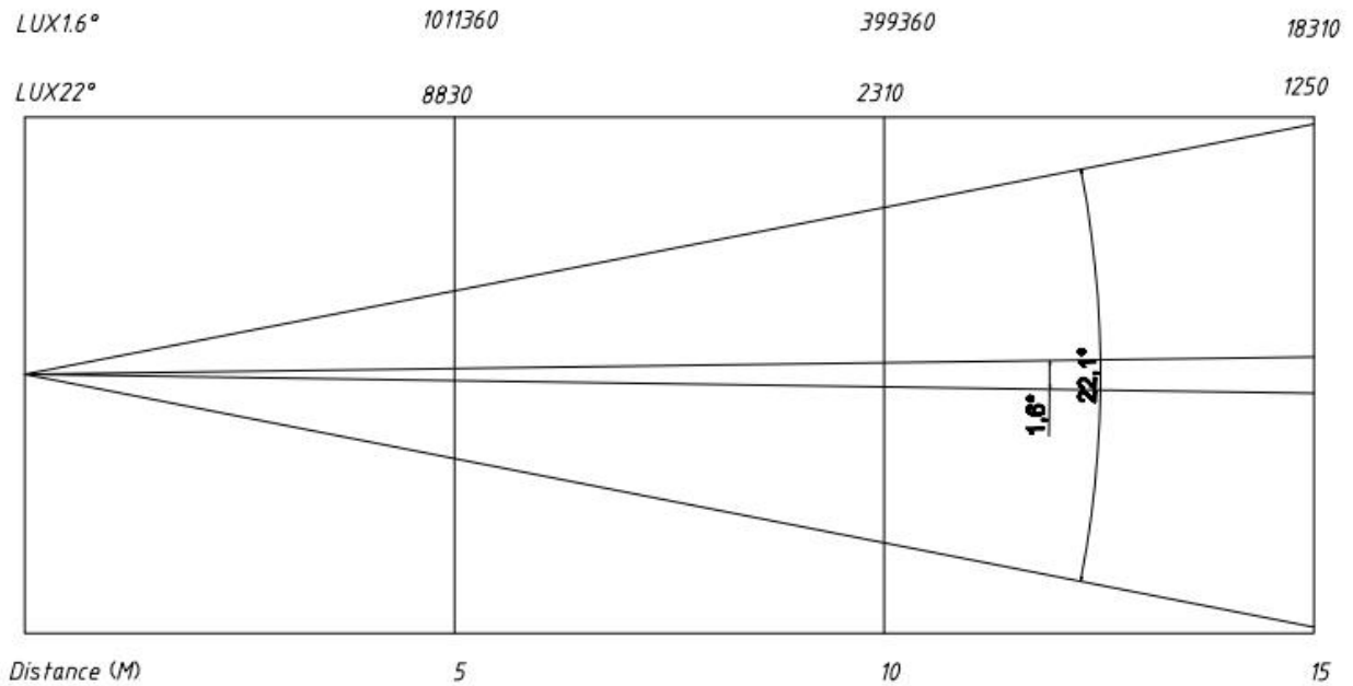
PHOTO METRICS DIAGRAM (Beam)
